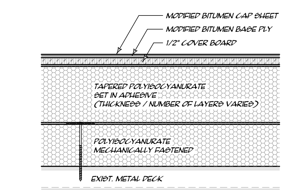
SECTION THRU ROOF ASSEMBLY ROOF SYSTEM NO. 2 2 R1 3" = 1'-0"
