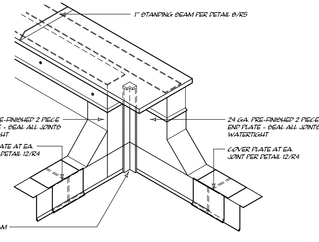
ISOMETRIC NET TO SCALE 8 STANDING SEAM JOINT RS NOT TO SCALE
