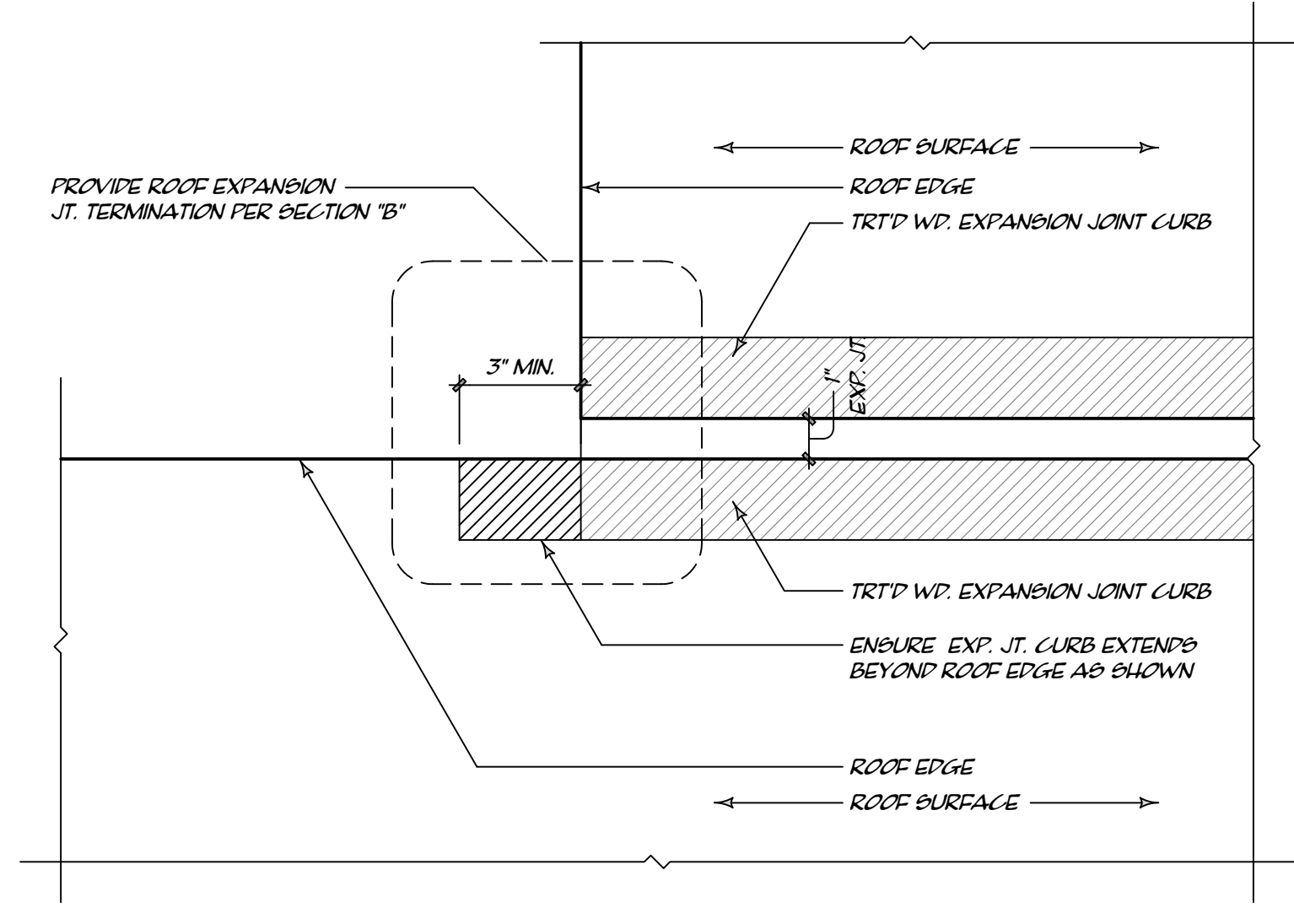
PLAN VIEW NET TO SCALE 7 ROOF TO ROOF EXP. JT. TERMINATION @ INSIDE CORNER RS 3" x 1'-0"
