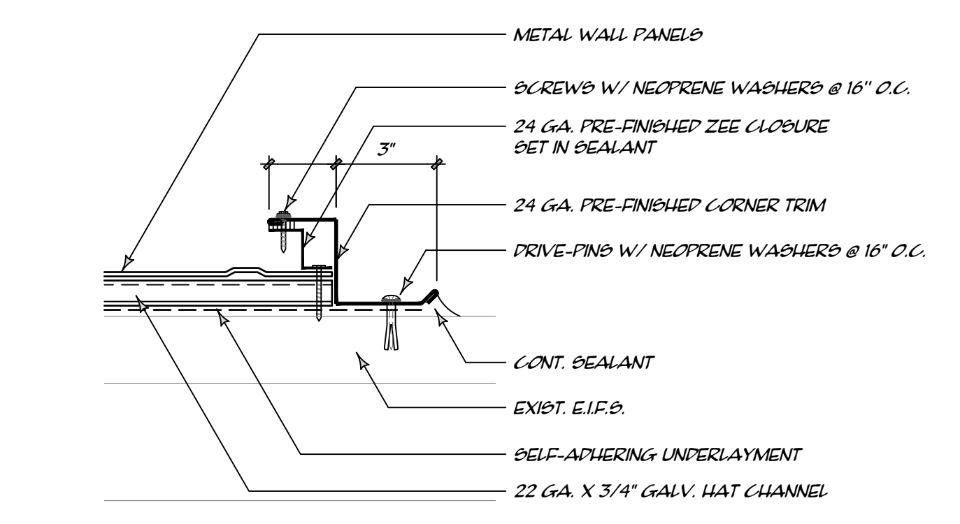
PLAN VIEW - WALL PANEL TERMINATION
