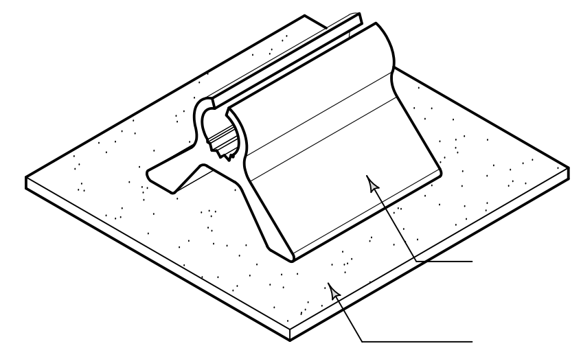
PIPE SUPPORT - ADJUSTABLE HEIGHT TYPE "A" RS 3" x 1'-0"
