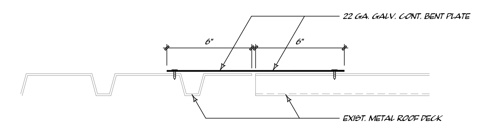
TRANSITION IN DECK RS 3" x 1'-0"
