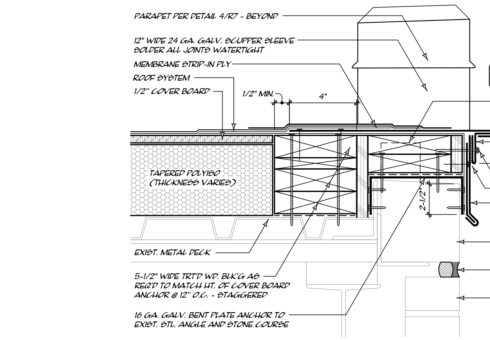
OVERFLOW SCUPPER
