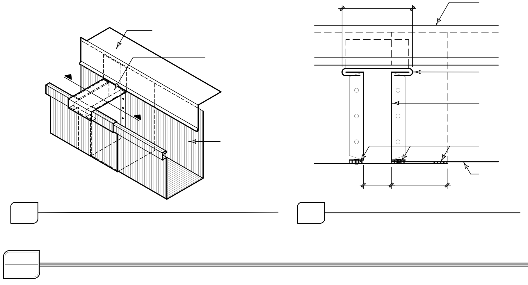
B SECTION NOT TO SCALE GUTTER JOINT
