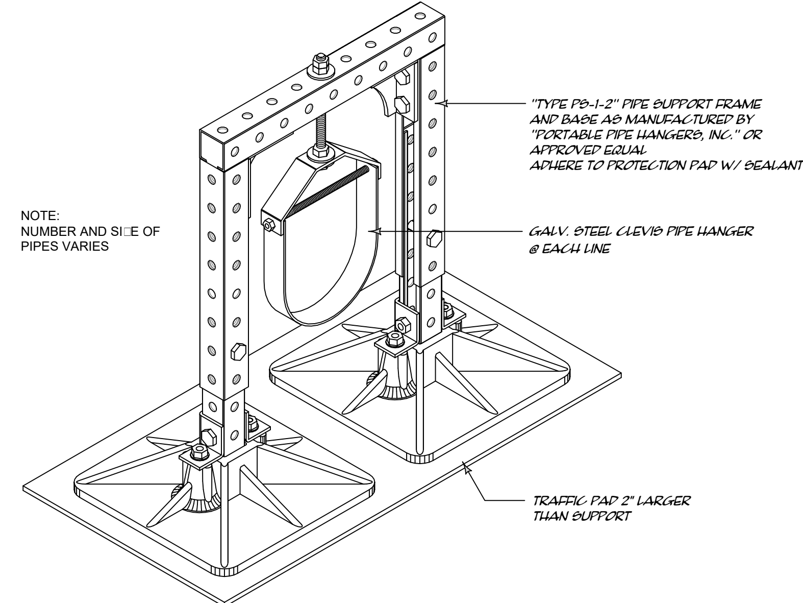
HANGING PIPE SUPPORT TYPE "C" RS NOT TO SCALE
