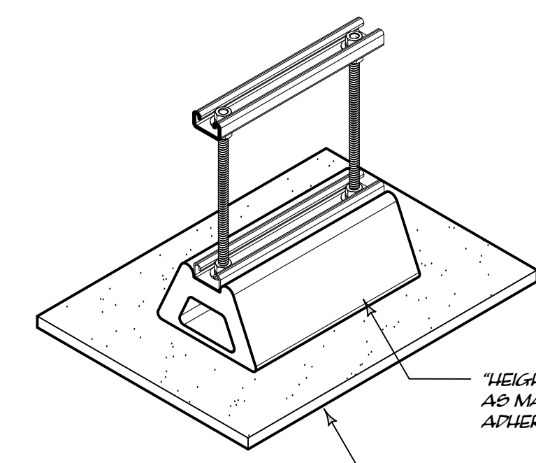
PIPE SUPPORT - ADJUSTABLE HEIGHT TYPE "B" RS 3" x 1'-0"
