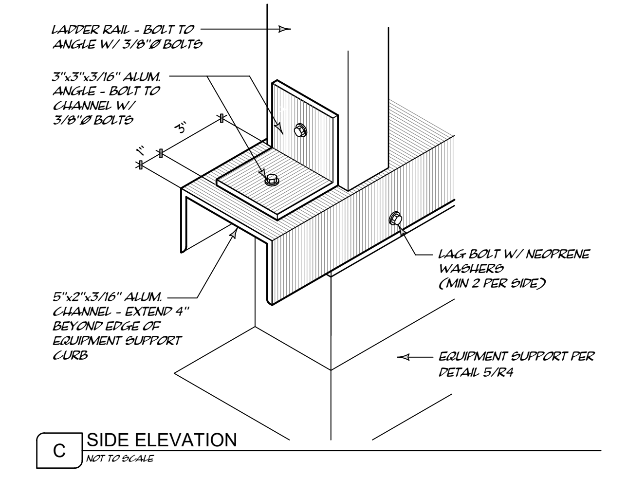
SIDE ELEVATION
