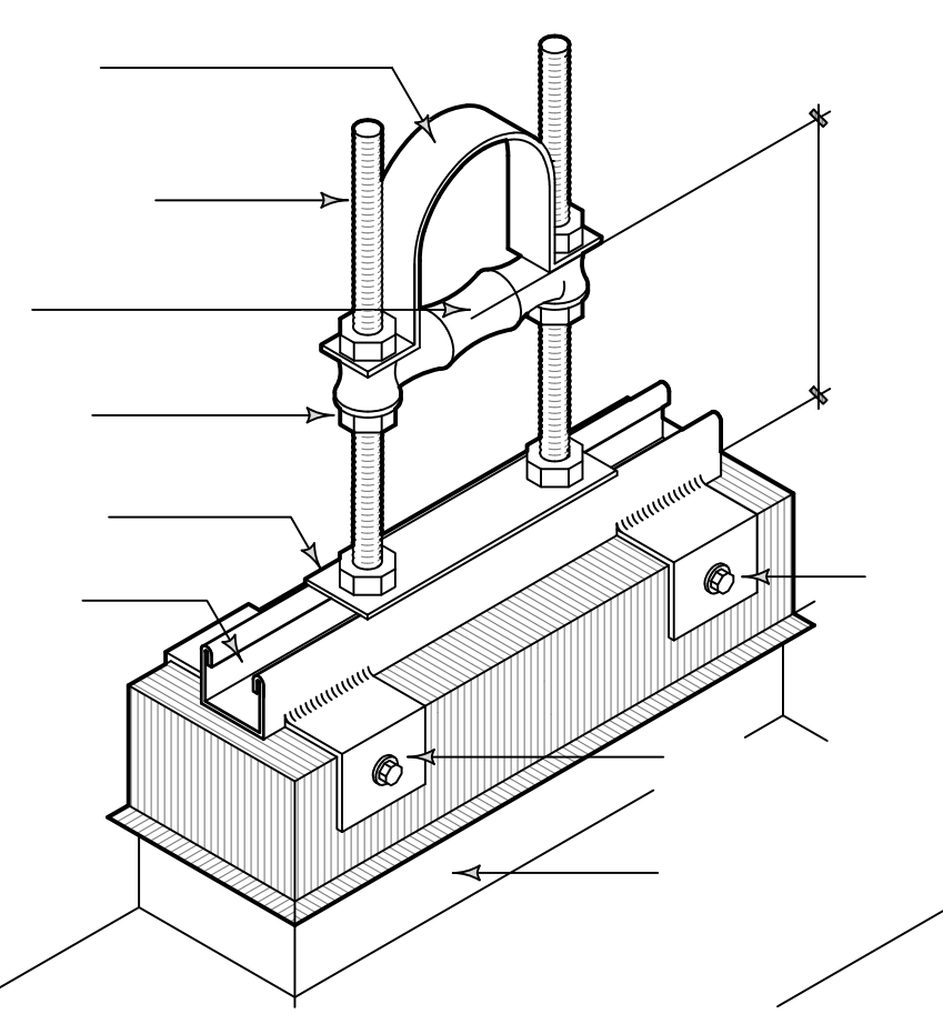
EXPANSION JOINT TERMINATION RS 3" x 1'-0"
