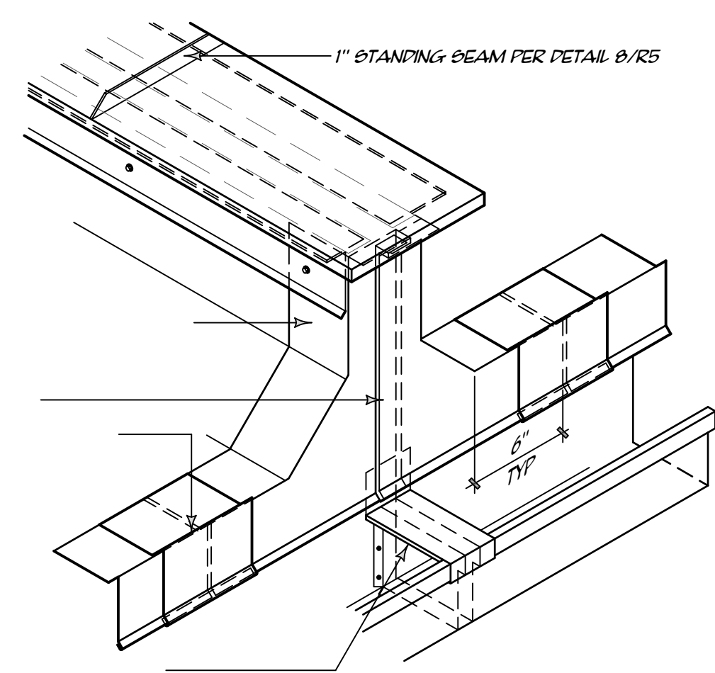
EXPANSION JOINT TERMINATION RS 3" x 1'-0"
